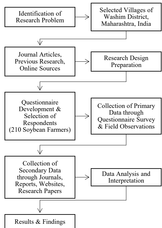
Figure 4 Methodology Flowchart
