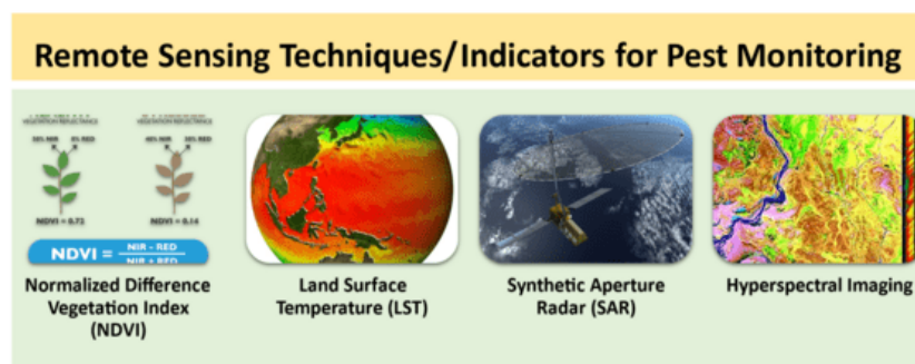
Fig. 2: Remote Sensing Techniques/Indicators for Pest Monitoring
