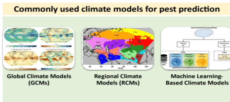
Fig. 1: Commonly used climate models for pest prediction
